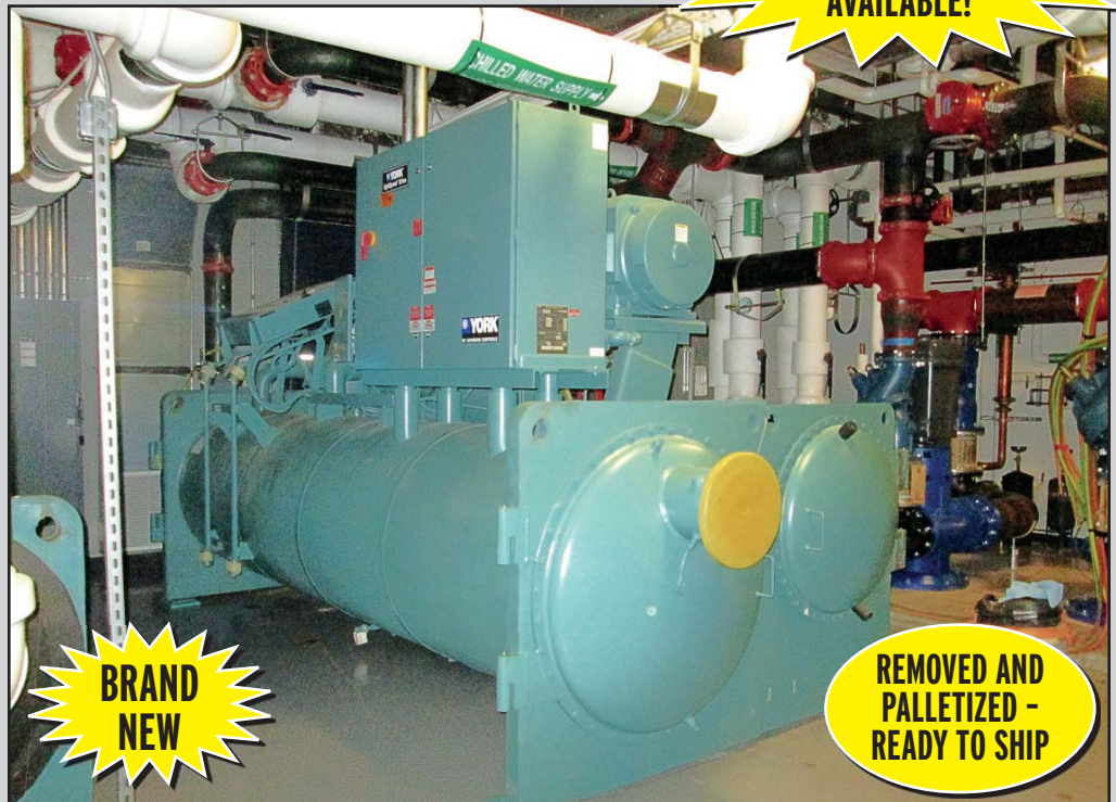
YORK 700-TON CENTRIFUGAL CHILLER
