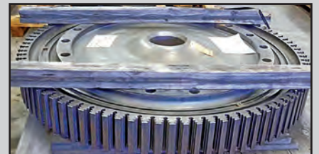
GE 7FA ROW 3 DISK (INCONEL 738)
