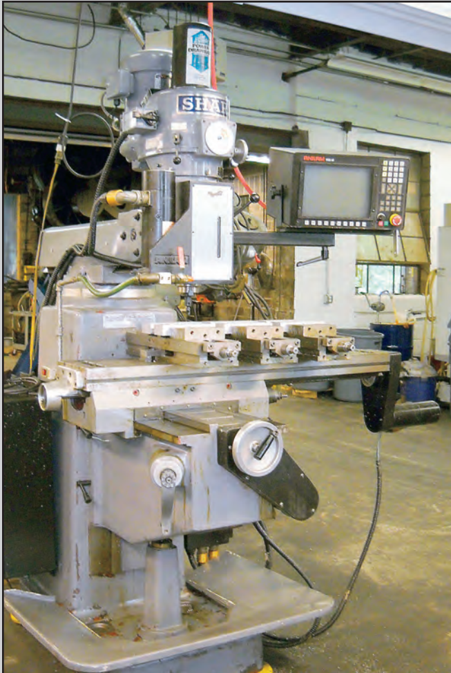
SHARP CNC VERTICAL MILL WITH POWER DRAW BAR
