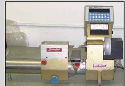
PRATT & WHITNEY SUPER MICROMETER
