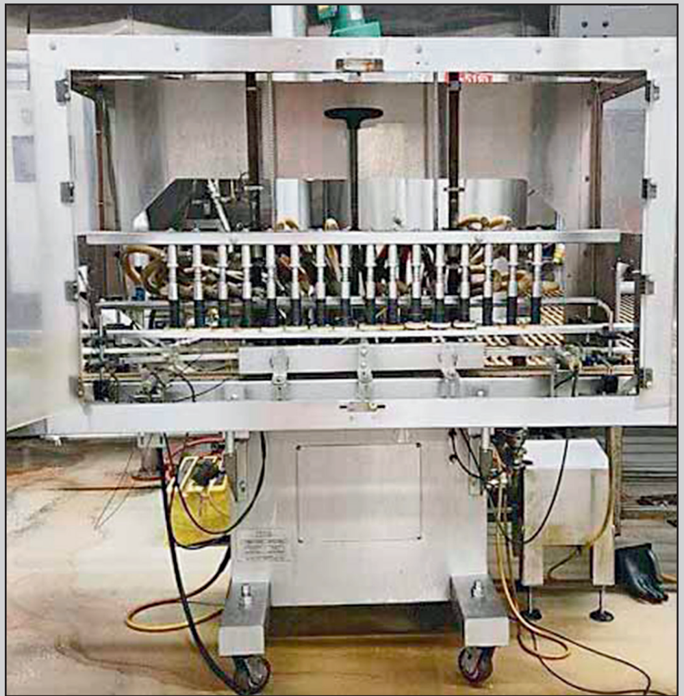
2019 ACASI GI 3300 14-VALVE IN-LINE BOTTLE FILLER
