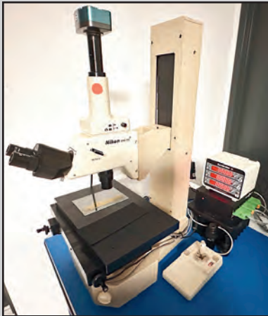
NIKON MM11-C MEASURING MICROSCOPE WITH 3-AXIS DRO
