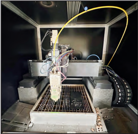
LASER BURNING TABLE WITH FSC-L II-VI LASER CUTTING HEAD
