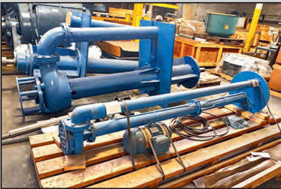
TOYO CANTILEVER SLURRY PUMPS
