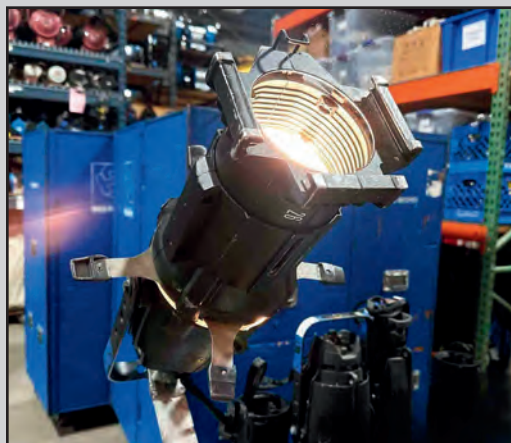
(SAMPLE) SOURCE 4ERS WITH 26 DEGREE LENS
